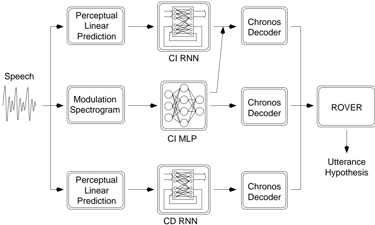
Figure 8: Schematic of the SPRACH Hub-4E Transcription System.
