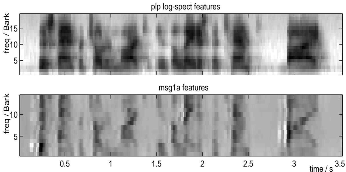
Figure 3: Comparison of spectrograms based on PLP and MSG processing, illustrating the effect of modulation-domain filtering. The vertical frequency axis is in Bark units; because the MSG features are based on signals bandlimited to 4 kHz, they extend only to 14 Bark, whereas the PLP features continue to 19 Bark.
