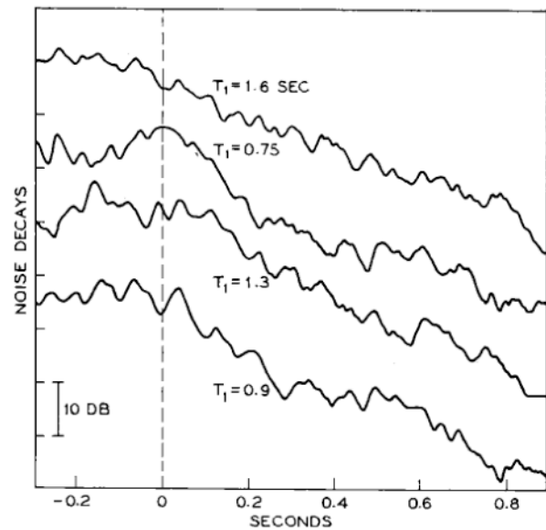
FIG. 1. Four noise-decay curves in Philharmonic Hall, New York (19 October 1963), obtained under identical conditions with \frac{1}{2} -oct band of noise centered at 167 cps. Noise source was near center stage, receiving point on Second Terrace (Seat A-221). Both loudspeaker and microphone had omnidirectional characteristics. The dashed vertical line indicates the time at which the noise signal was switched off. Note the large differences in the four decay curves that result from the randomness of the excitation signal. The values of T_1 are reverberation times based on straight-line fits to the first 10 dB of the decays.
